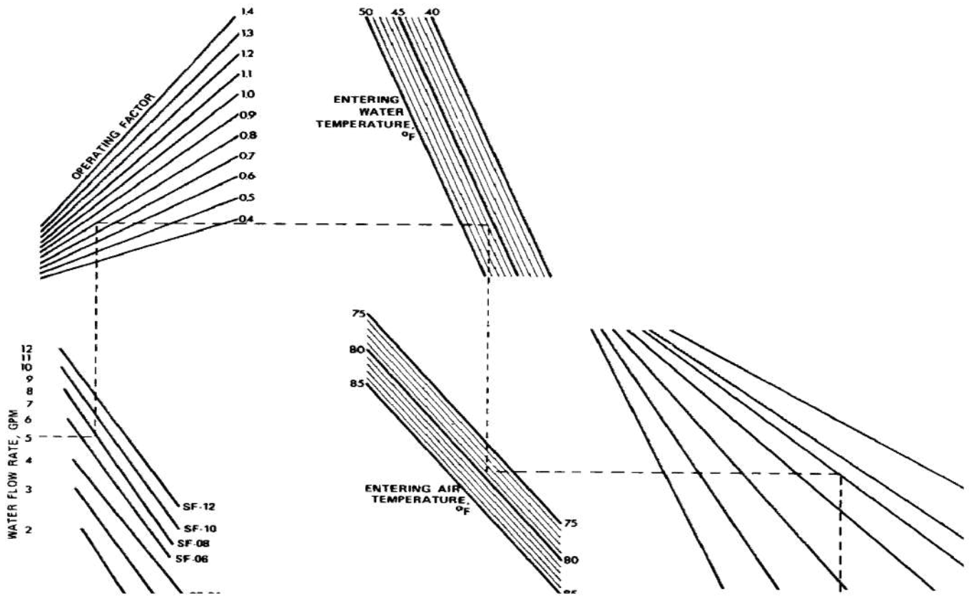
FIGURE 1. WET TARING SENSIBLE COOLING CAPACITY
