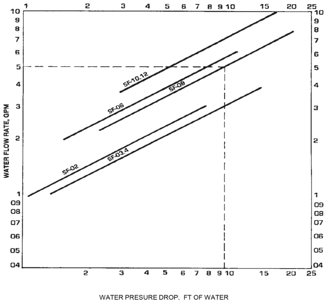
FIGURE 5. THE COIL PRESSURE DROP
